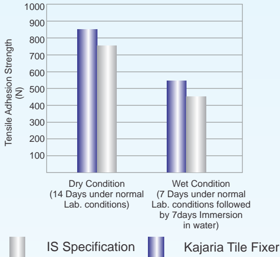
Comparison of Kajaria Adhesive with IS Specification
