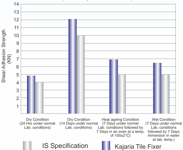
Comparison of Kajaria Adhesive with IS Specification
